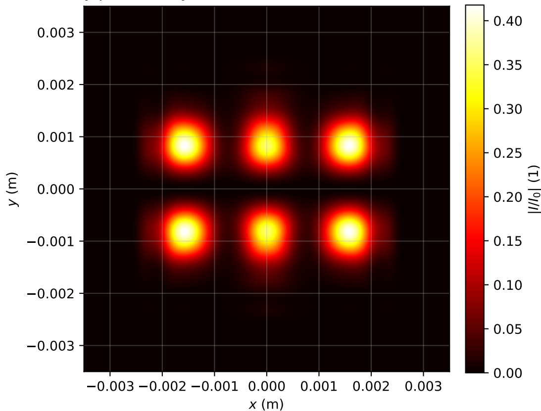
Intensity profile I(x, y, z = 3.423)/I_0 , P_{in}=3.0P_{cr} , artificial time
